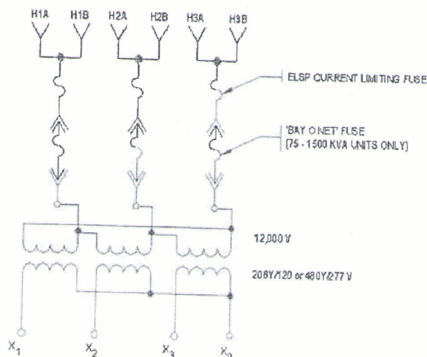
Figure 2 Internal Schematic
